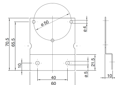
Mounting bracket 6402
