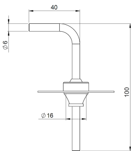
Duct connection for Climaset® 6550/6556
