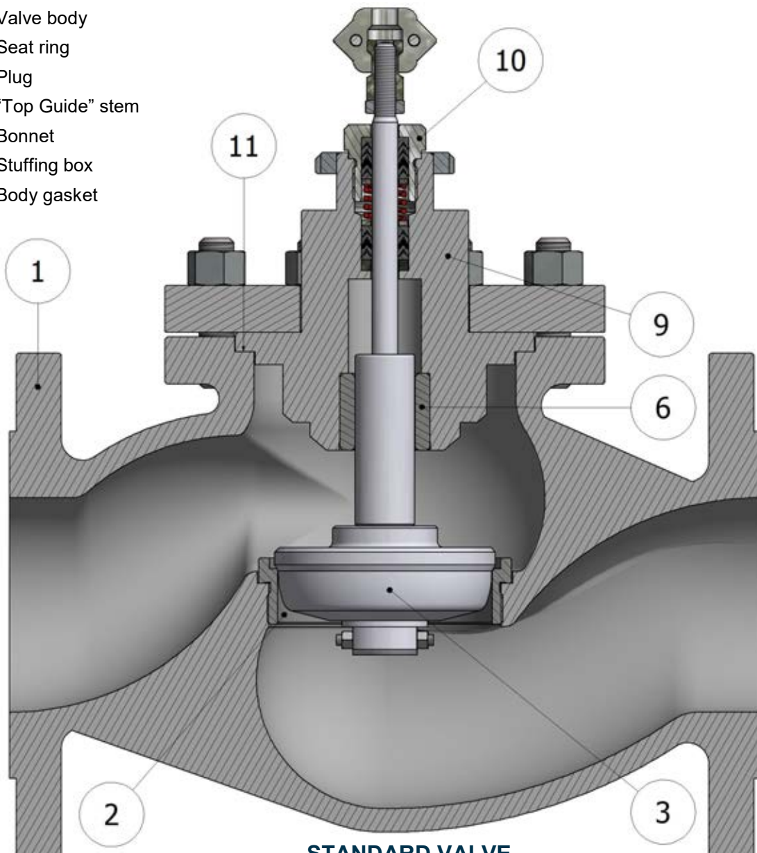
STANDARD VALVE
